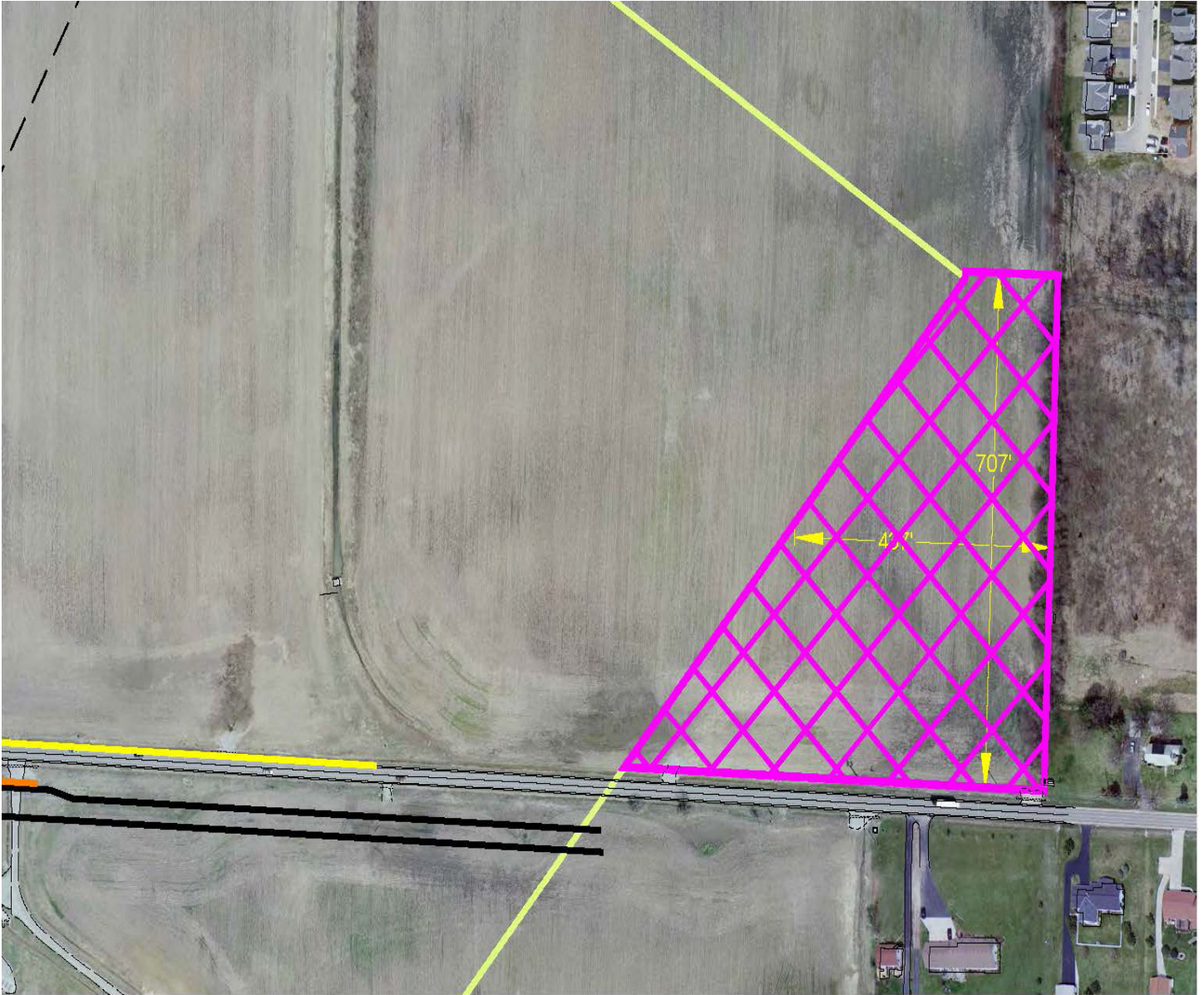
Alkire Road -- Parcel #1B 7 Ac. ± 1" = 200'
